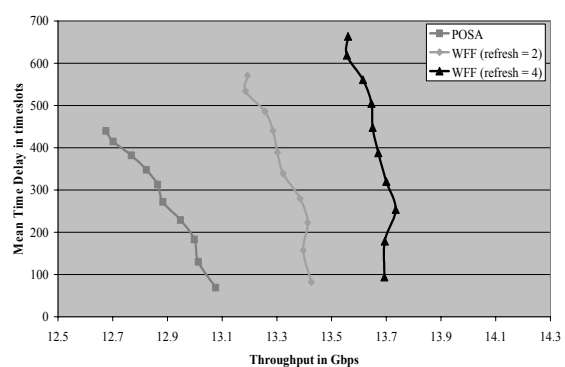
Fig.7. Throughput vs. Mean Time Delay ( W = 3 )
