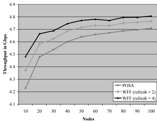
Fig.4. Network Throughput ( W = 2 )
