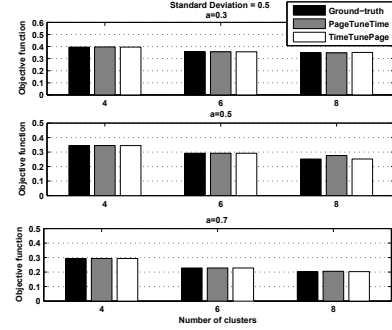
(b) Objective function values as a function of the number of clusters
