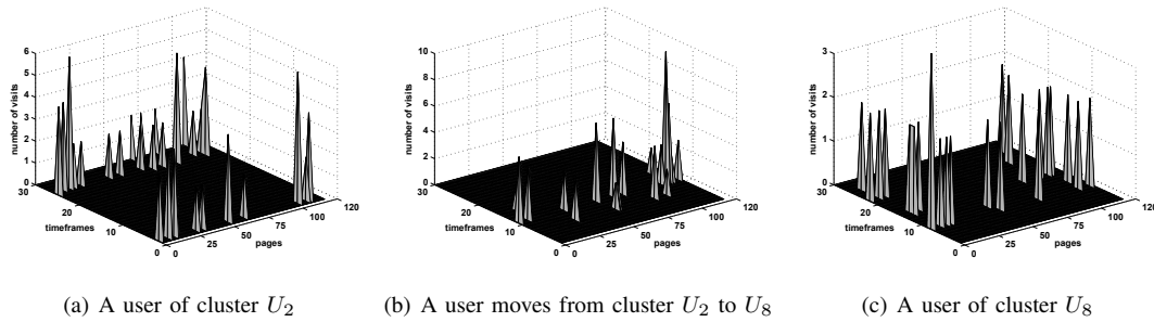
Fig. 7. The PAGETUNETIME algorithm: the impact of the time aspect in a user's reassignment.
